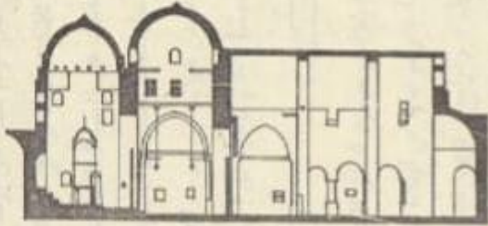
SECTION AB
